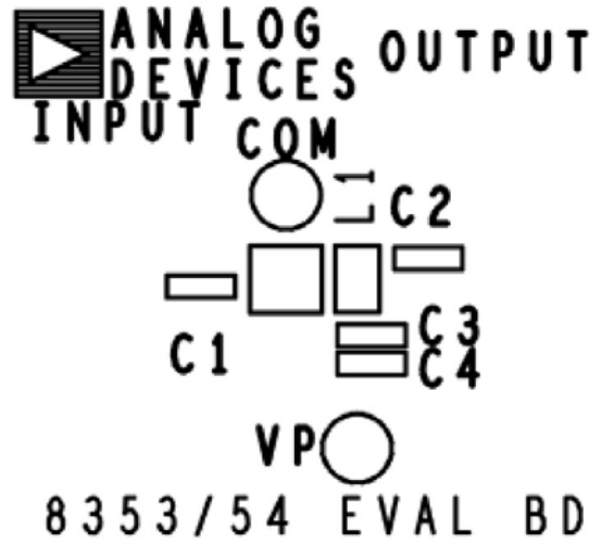
Figure 41. Silkscreen Top
